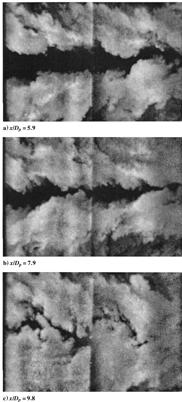
Fig. 8 PLIF image for the air jet of case A2.
