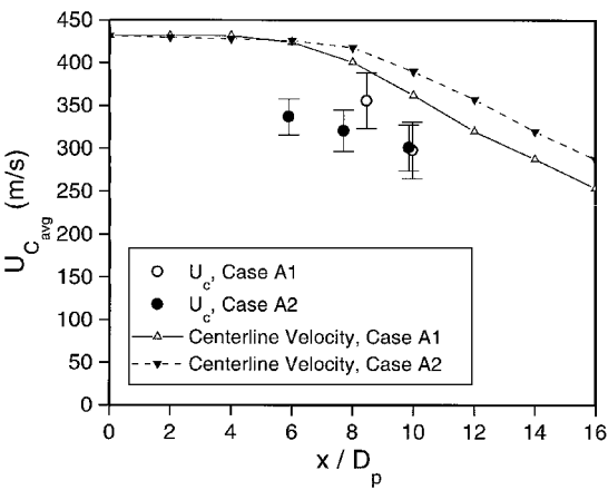
Fig. 10 Ensemble-averaged convective velocities vs axial distance for the air jets. The mean centerline velocity distributions are also shown.
