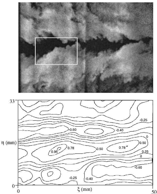
Fig. 9 PLIF image and cross correlation for the air jet of case A2, where x/D_p = 7.9 and \Delta t = 80 \theta s .
