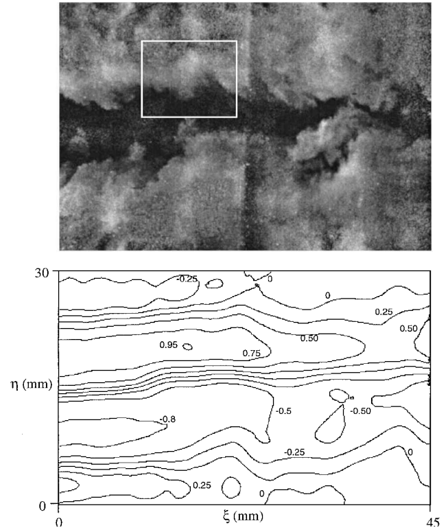
Fig. 13 PLIF image and cross correlation for the helium-air jet of case C at x/D_p = 5.7 . The new mass of fluid in the delayed sheet results in a poor correlation and rejection of this measurement.
